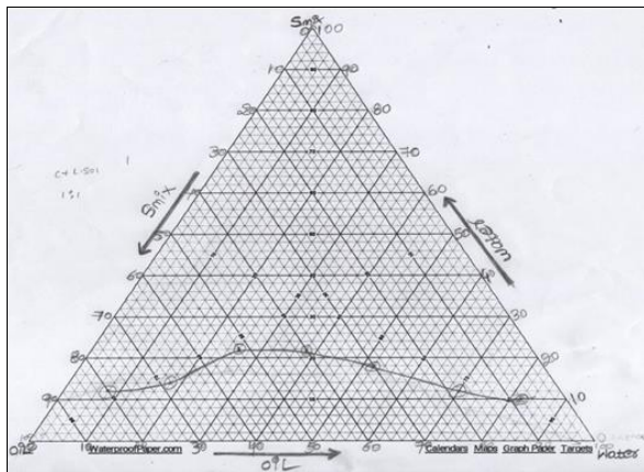
Fig 3 (a): Ternary phase diagram of 1:1 ratio of coconut oil: S mix (labrasol: PEG 400) and water
