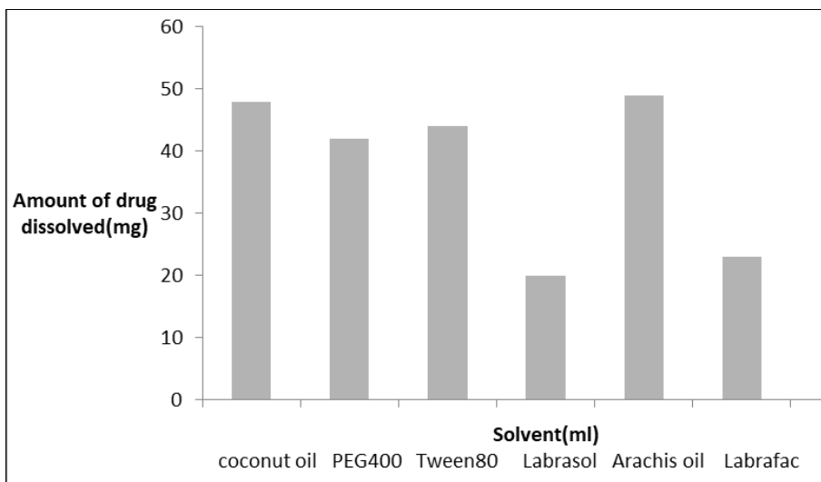
Fig 1: Solubility profile of Febuxostat in various surfactant and co-surfactant
