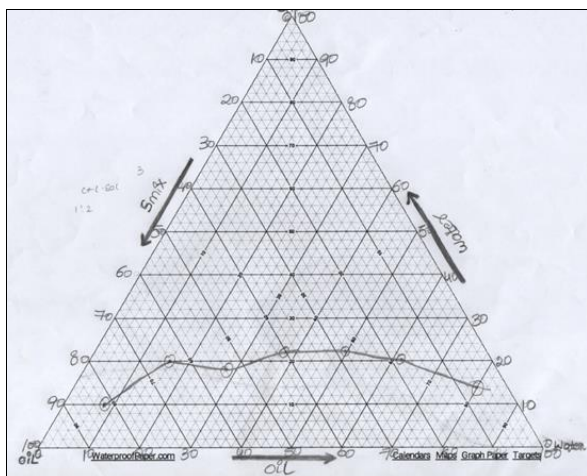
Fig 3(b): Ternary phase diagram of 1:2 ratio of coconut oil: s mix (labrasol: PEG 400) and water
