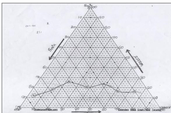
Fig 3(c): Ternary phase diagram of 2:1 ratio of coconut oil: s mix (labrasol: PEG 400) water
